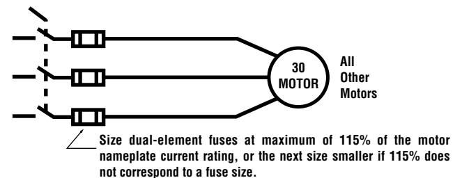
Figure 6B. All Other Motors (Over 40°C or Less Than 1.15 S.F.)
