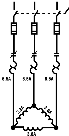
Figure 4C. Delta-connected three-phase motor loaded to only 65% of its rated horsepower. Normal FLA = 10 amperes. Overload (overcurrent) protection should be based upon the motor's actual current draw for the underloaded situation for optimum protection. If load varies, overload protection is difficult to achieve. Temperature sensors, phase failure relays and current differential relays should be installed.
