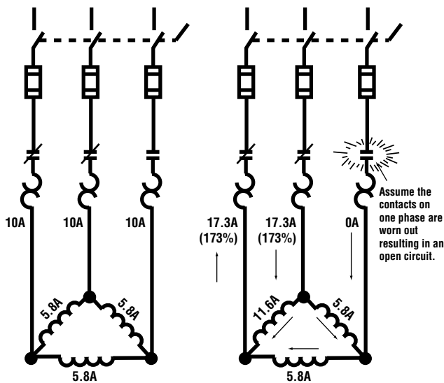
Delta-Connected Motor FLA = 10 Amperes
