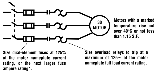
Figure 7A. 40°C or 1.15 S.F. Motors
