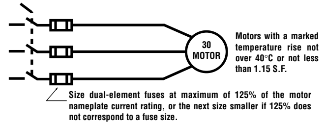
Figure 6A. 40°C or 1.15 S.F. Motors
