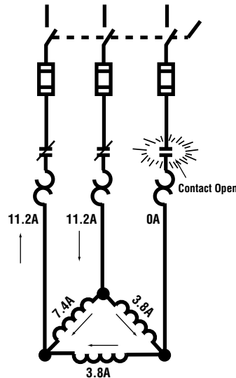
Figure 4C. Delta-connected three-phase motor loaded to only 65% of its rated horsepower. Normal FLA = 10 amperes. Overload (overcurrent) protection should be based upon the motor's actual current draw for the underloaded situation for optimum protection. If load varies, overload protection is difficult to achieve. Temperature sensors, phase failure relays and current differential relays should be installed.
