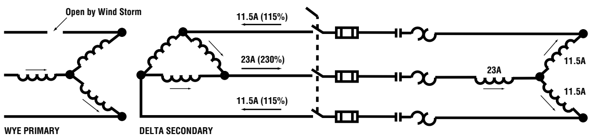
Figure 5B. (Wye-Connected Motor) Diagram showing how the phase currents to a three-phase motor increase when a single-phasing occurs on the primary. For older installations where the motor is protected by two overload devices, the phase winding having the 230% current will burn up. However, properly sized overload relays or LOW-PEAK® or FUSETRON® dual-element, time-dealy fuses will clear the motor from the power supply.
