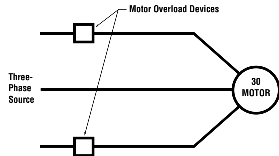
Figure 1. Diagram showing two overload devices protecting a three-phase motor. This was acceptable by the National Electrical Code prior to 1971.
