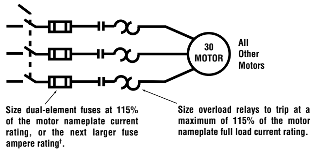
Figure 7B. All Other Motors (Over 40°C or Less Than 1.15 S.F.)
