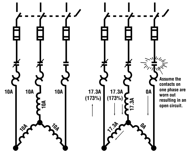
WYE-Connected Motor FLA = 10 Amperes
