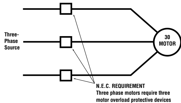
Figure 3. Since 1971, The National Electrical Code has required three overload protective devices for the protection of three-phase motors, one in each phase.
