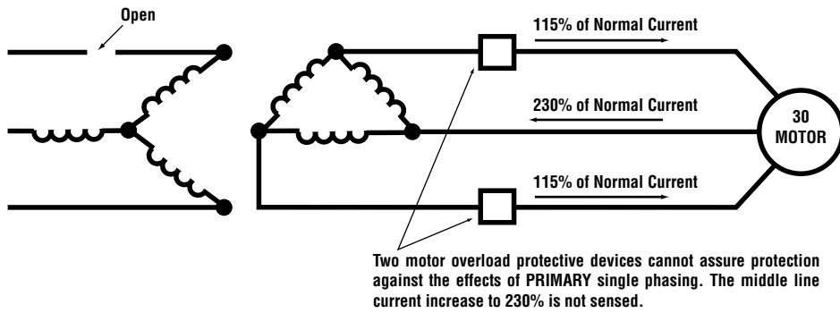
Figure 2. Diagram of a WYE/DELTA transformation with one primary phase open. The motor is protected by two overload devices. Note that one phase to the motor is carrying two times that of the other two phases. Without an overload device in the phase that is carrying two times the current in the other two phases, the motor will burn out.
