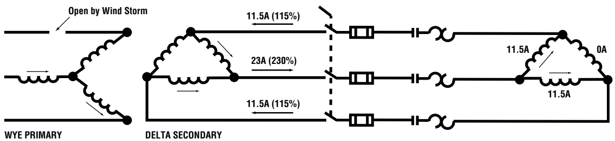
Figure 5A. (Delta-Connected Motor) Diagram showing how the phase currents to a three-phase motor increase when a single-phasing occurs on the primary. For older installations where the motor is protected by two overload devices, the phase winding having the 230% current will burn up. However, properly sized overload relays or LOW-PEAK® or FUSETRON® dual-element, time-dealy fuses will clear the motor from the power supply.
