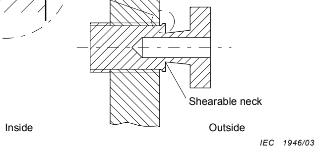
Figure 22 – Examples of closing devices for unused apertures
