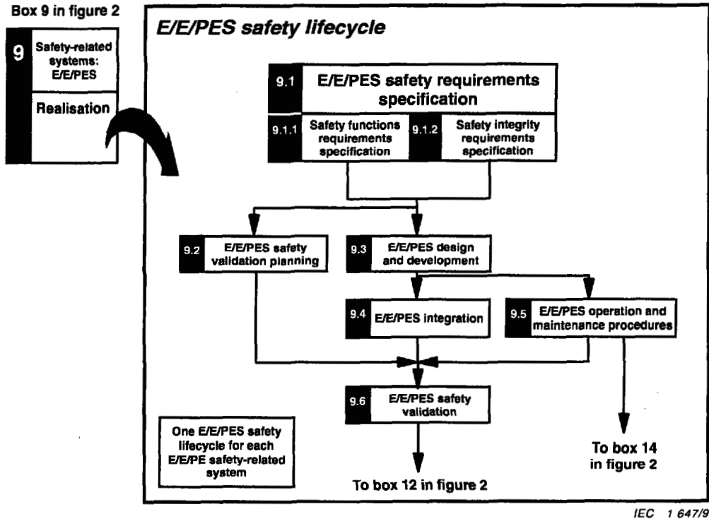
Figure 3 — E/E/PES safety lifecycle (in realisation phase)
