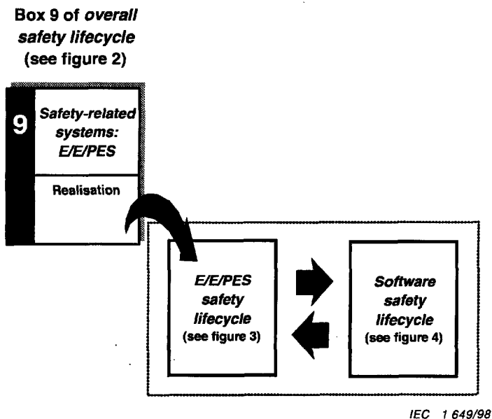
Figure 5 – Relationship of overall safety lifecycle to E/E/PES and software safety lifecycles
