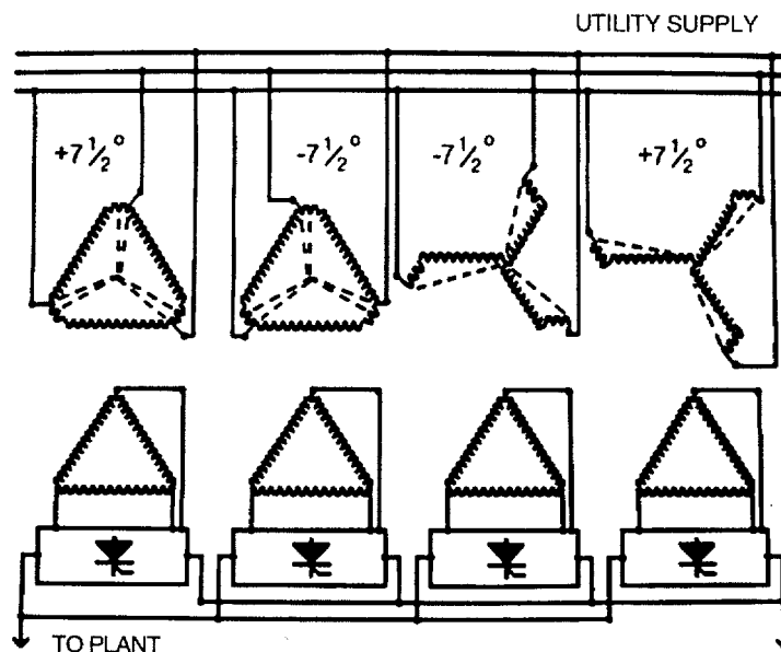
Figure 7-11—Transformer Connections for a 24-Pulse System
