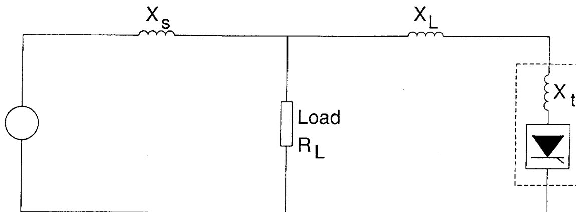
Figure 8-6—Impedance Diagram
