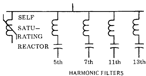
Figure 7-9—Reactive Power Compensation Using Saturable Reactor
