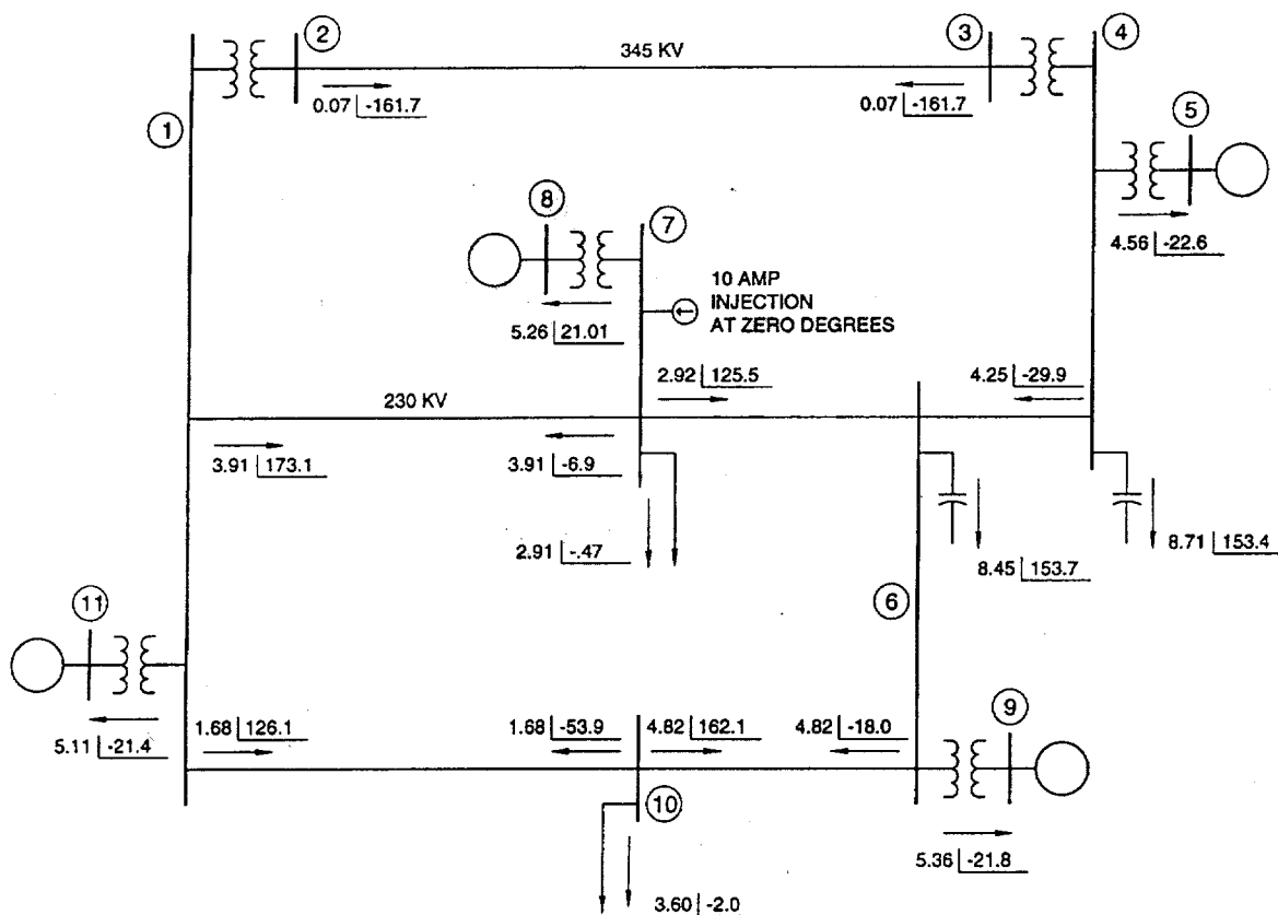
Figure 5-8—Fifth Harmonic Current Flowing in a Transmission Network due to a 10 A Injection at Bus 7
