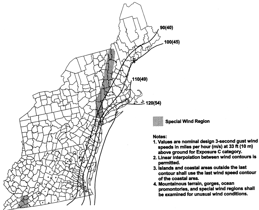
Fig 250-2(e) Mid and Northern Atlantic Hurricane Coastline*
