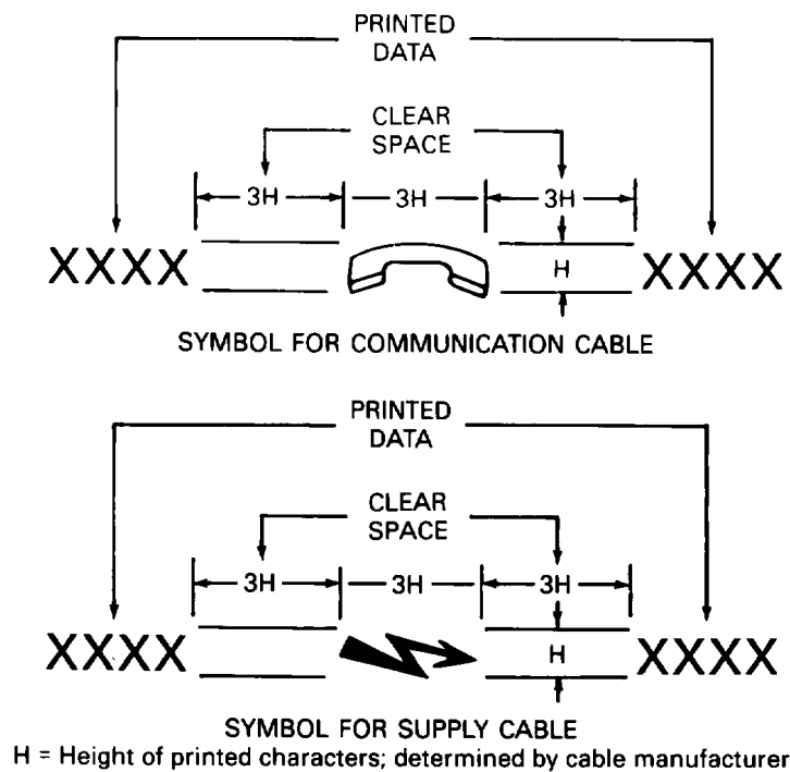
Fig 350-1 Symbols for Identification of Buried Cables
