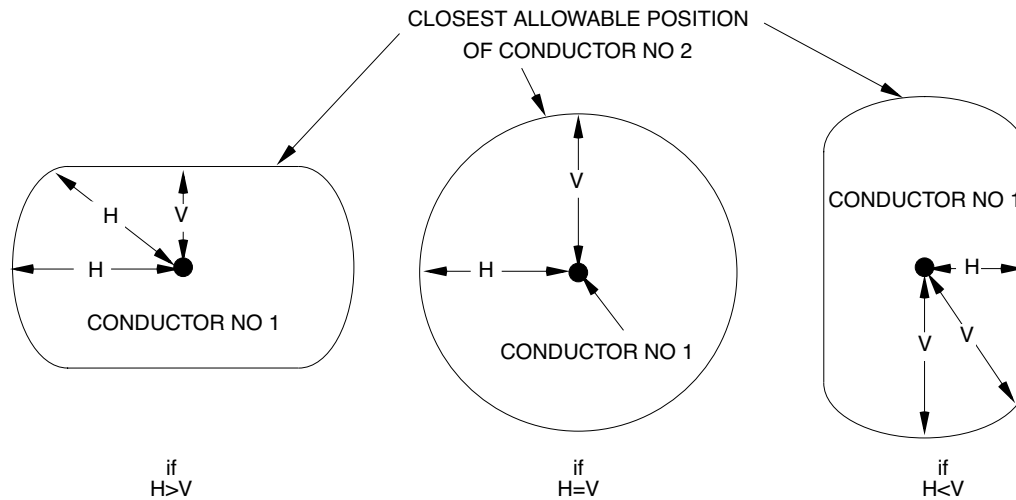
Fig 233-3 Clearance Envelope
