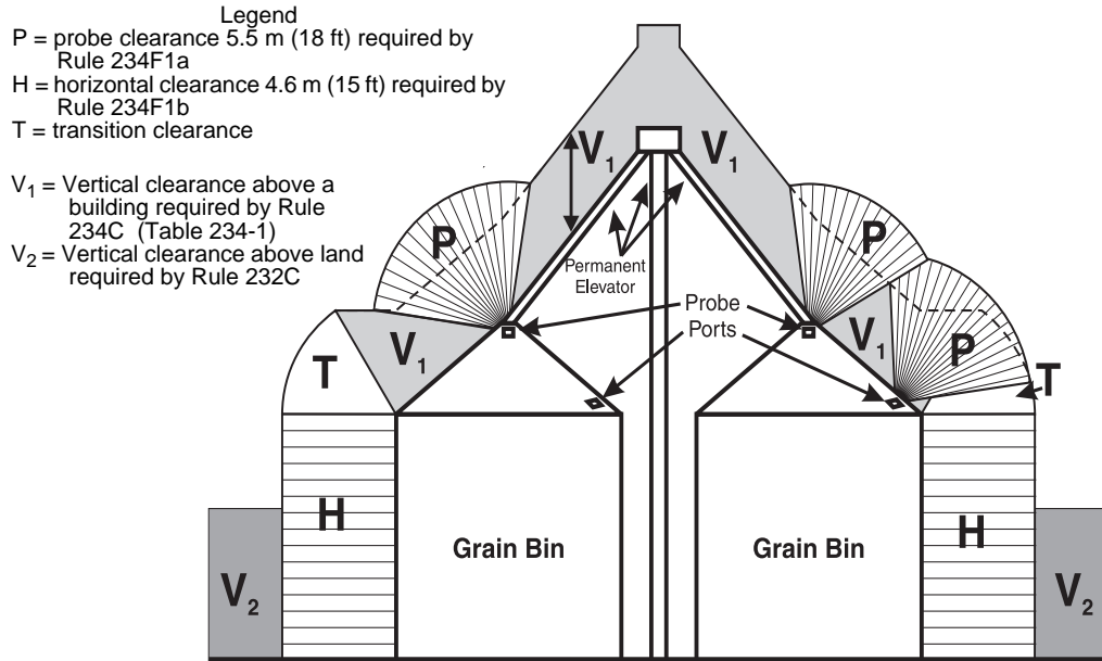
Fig 234-4(a) Clearance Envelope for Grain Bins Filled by Permanently Installed Augers, Conveyors, or Elevators
