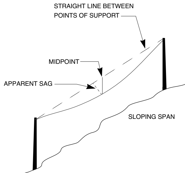
Fig D-1 Sag and Apparent Sag
