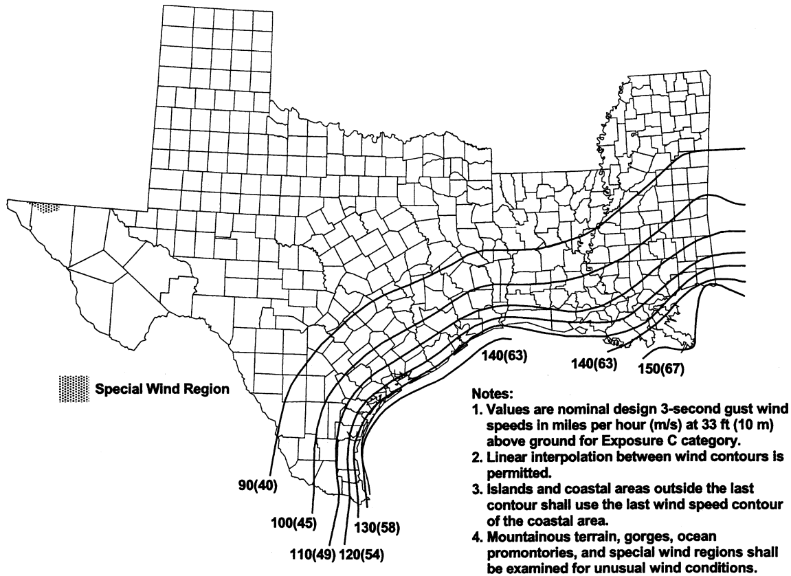
Fig 250-2(c) Western Gulf of Mexico Hurricane Coastline*
