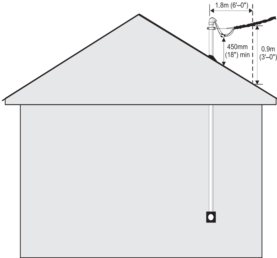
Elevation View
