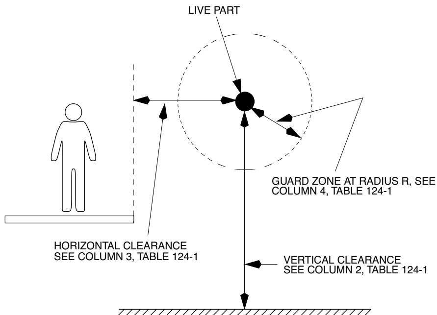
Fig 124-1 Clearance From Live Parts
