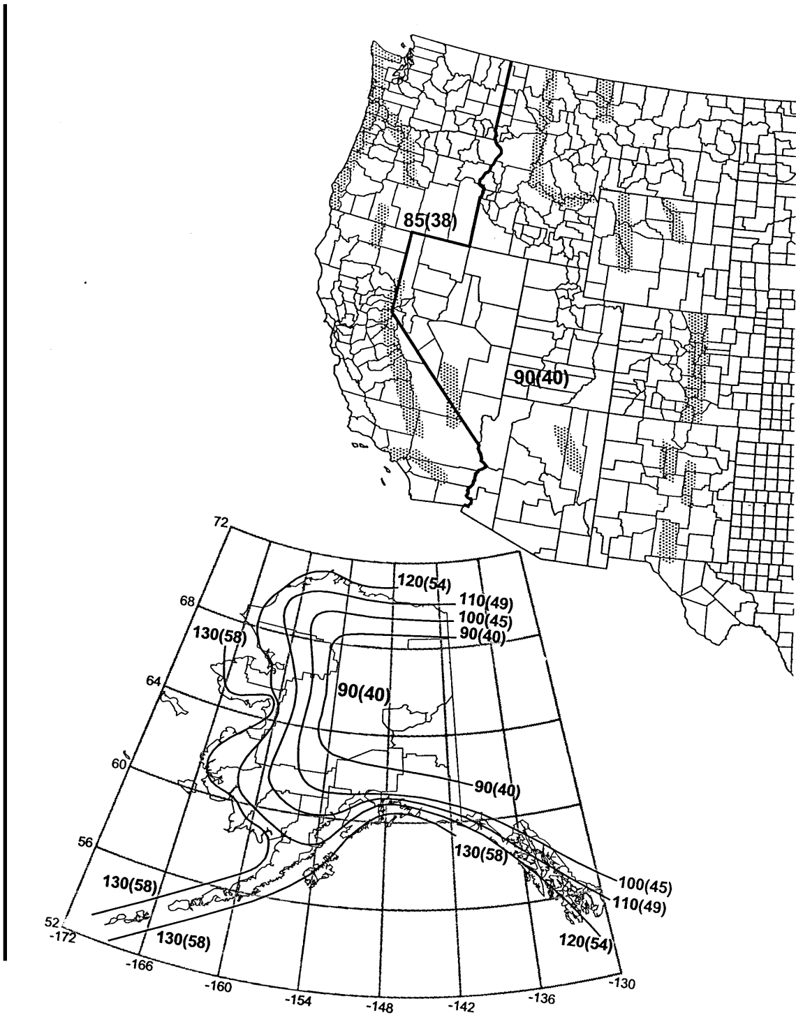
Fig 250-2(a) Basic Wind Speeds*
