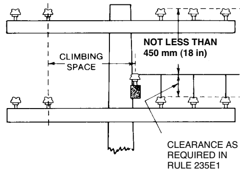
Fig 237-1 Obstruction of Working Space by Buckarm
