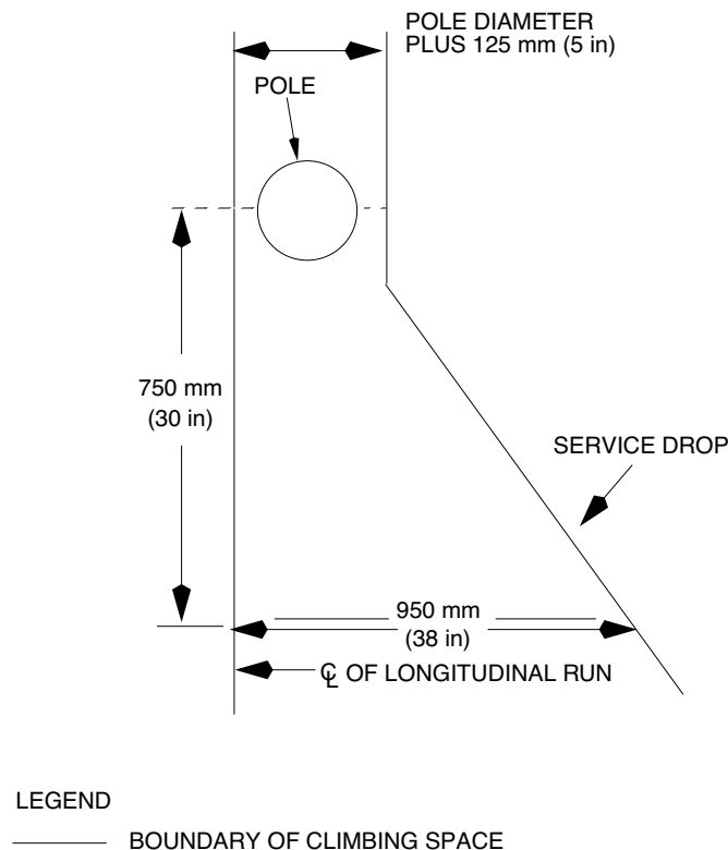
Fig 236-1 Rule 236G, Exception 3
