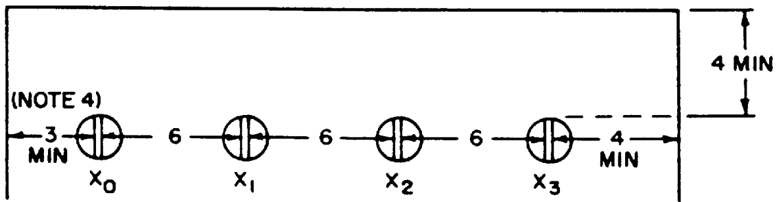
(b) In-Line Low-Voltage Terminal Arrangement
