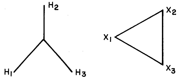
Fig. 3 Y-Δ Connection
