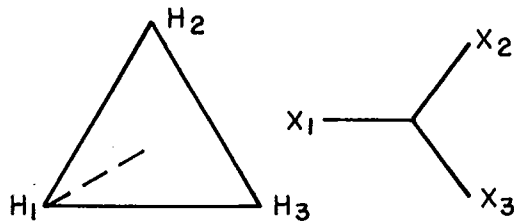
Δ-Y Connection (b)
