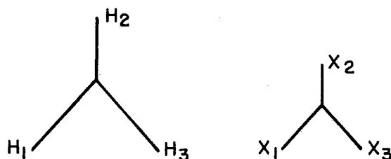
Fig. 4 Y-Y Connection
