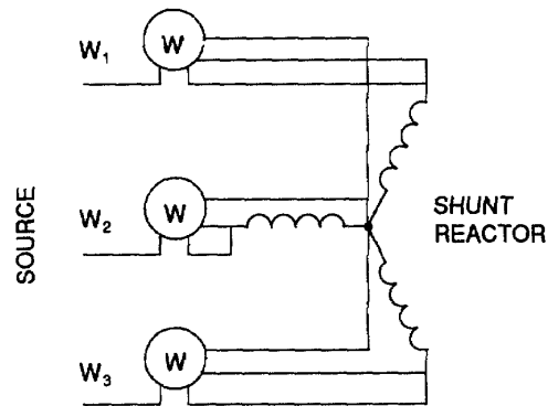
Figure 5—Three-Wattmeter Method with Shunt Reactor Neutral Available
