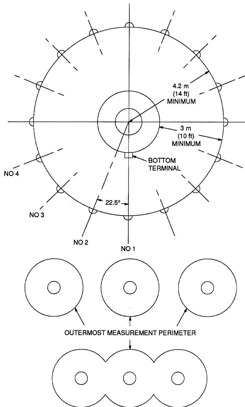
Figure 8—Microphone Locations for Audible-Sound Tests of Dry-Type Shunt reactors
