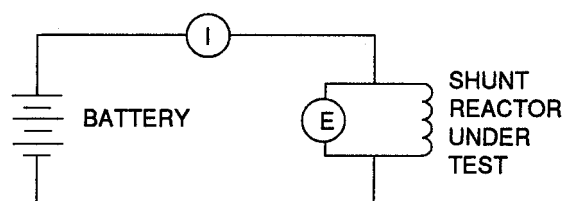
Figure 2—Connections for the Drop-of-Potential Method of Resistance Measurement
