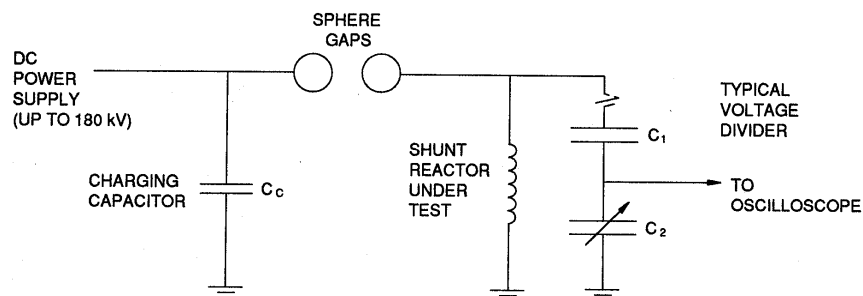
Figure 3.A Turn-to-Turn Test Circuit
