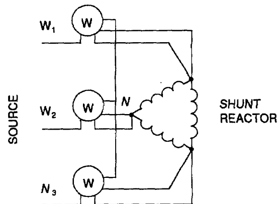
Figure 6—Three-Wattmeter Method Using Artificial Wattmeter Neutral N
